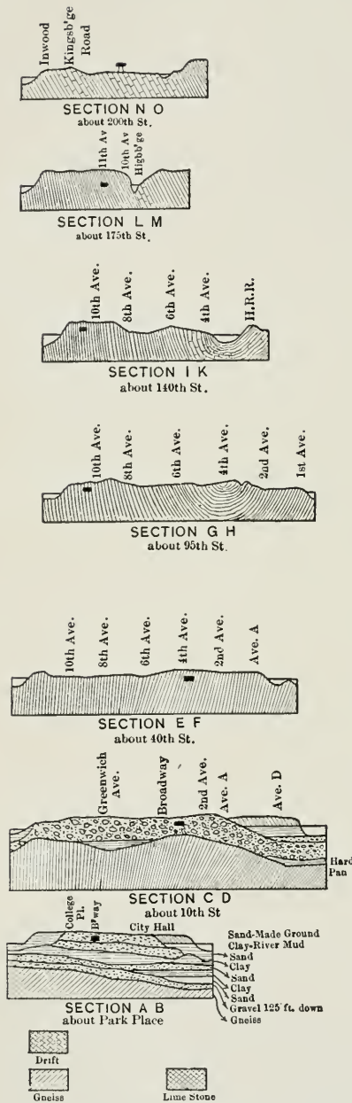
Cross-sections of Manhattan Island, showing Geological Formations.
